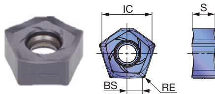
PNCU0905-W (Right hand)
